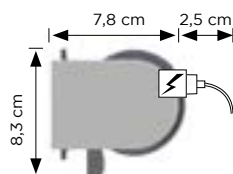
Wandmontage
